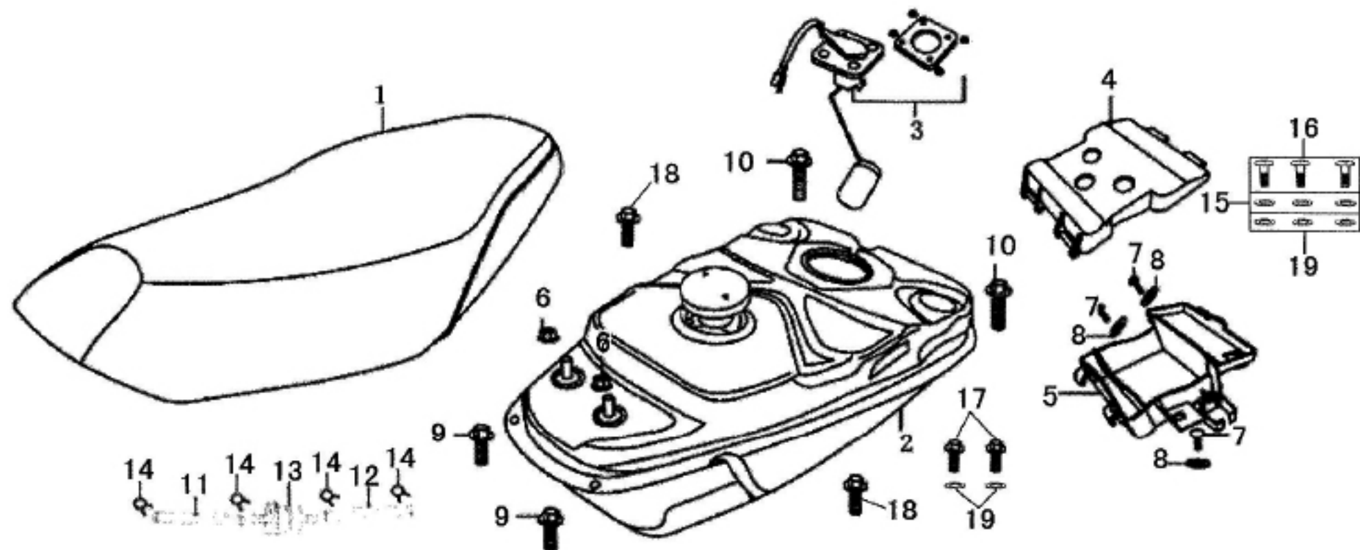
F-6 座垫 油箱 SEAT & FUEL TANK
