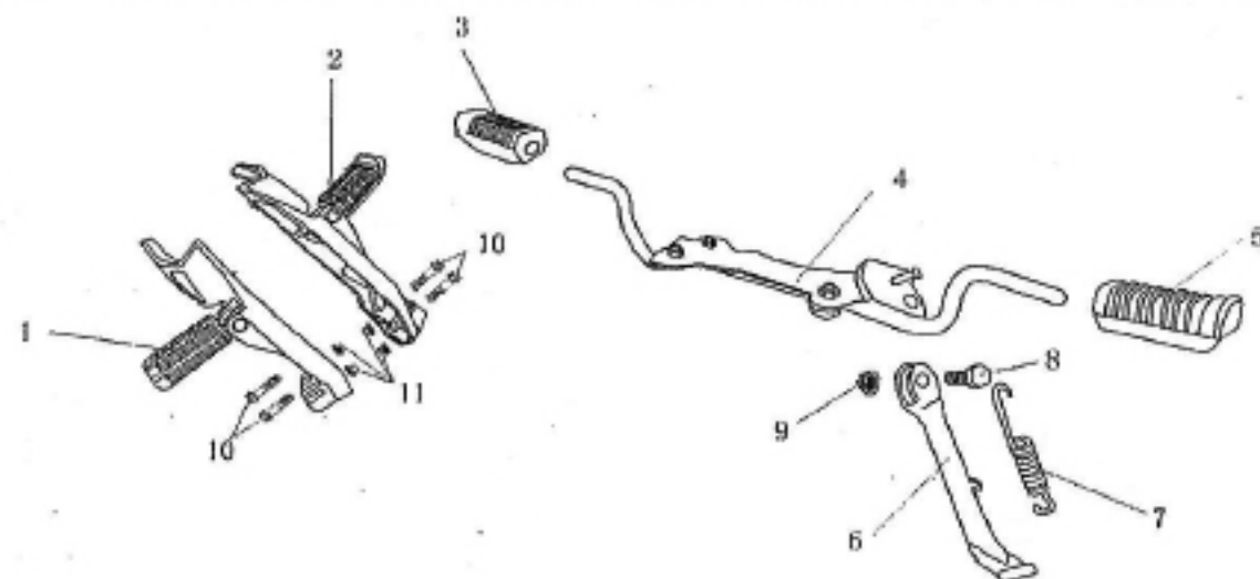
F-18 脚踏 PEDAL
