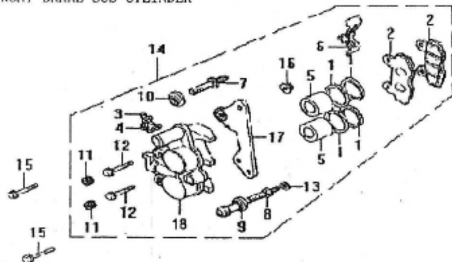
F-8 前制动分泵 FRONT BRAKE SUB-CYLINDER
