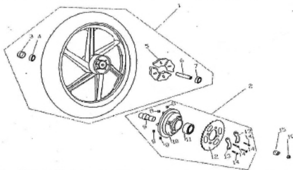
P-14 后轮 REAR WHEEL
