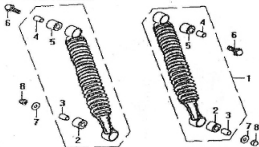
F-16 后减震器 REAR SHOCK ABSORBER
