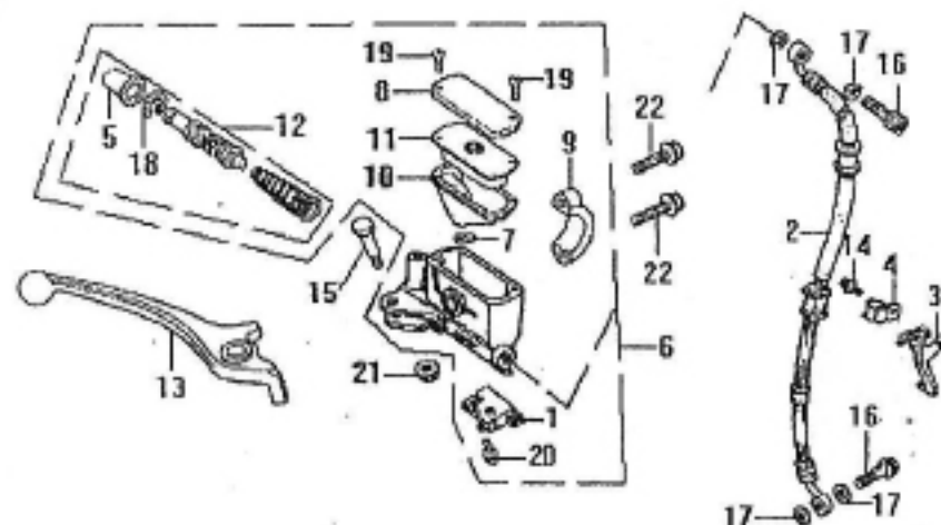
FRONT BRAKE MAIN CYLINDER
