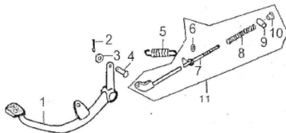
F-17 后制动踏板 REAR BRAKE PEDAL ASSY
